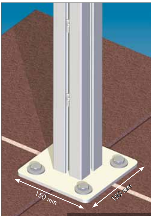
Plaque de sol – montant
